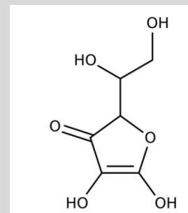
structure ascorbic acid
