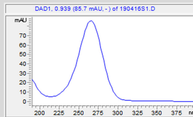
Spectral data of vitamin C
