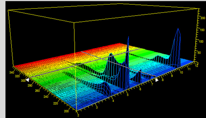
Amino acid ultra violet spectrum
